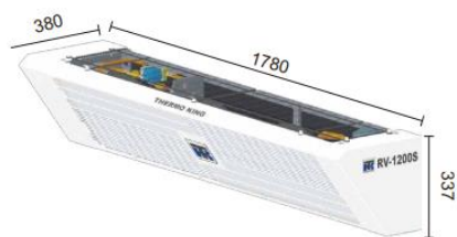
RV-1000/1100/1200S Condenser
