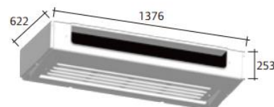
RV-1000S Evaporator
